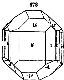
Norwich, Ct.
